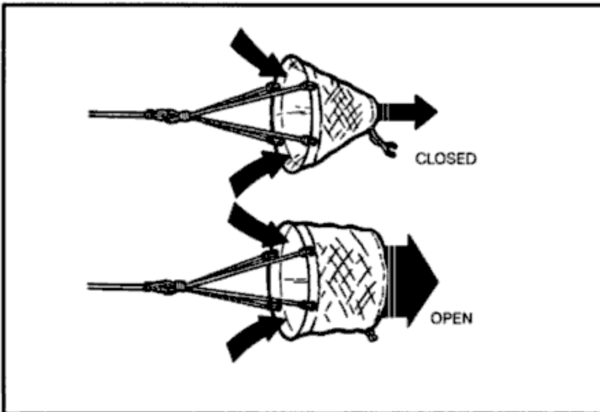
Figure 16-5. Sea anchor.
